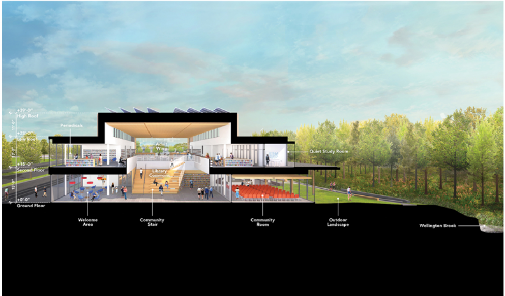
TRANSVERSE SECTION
