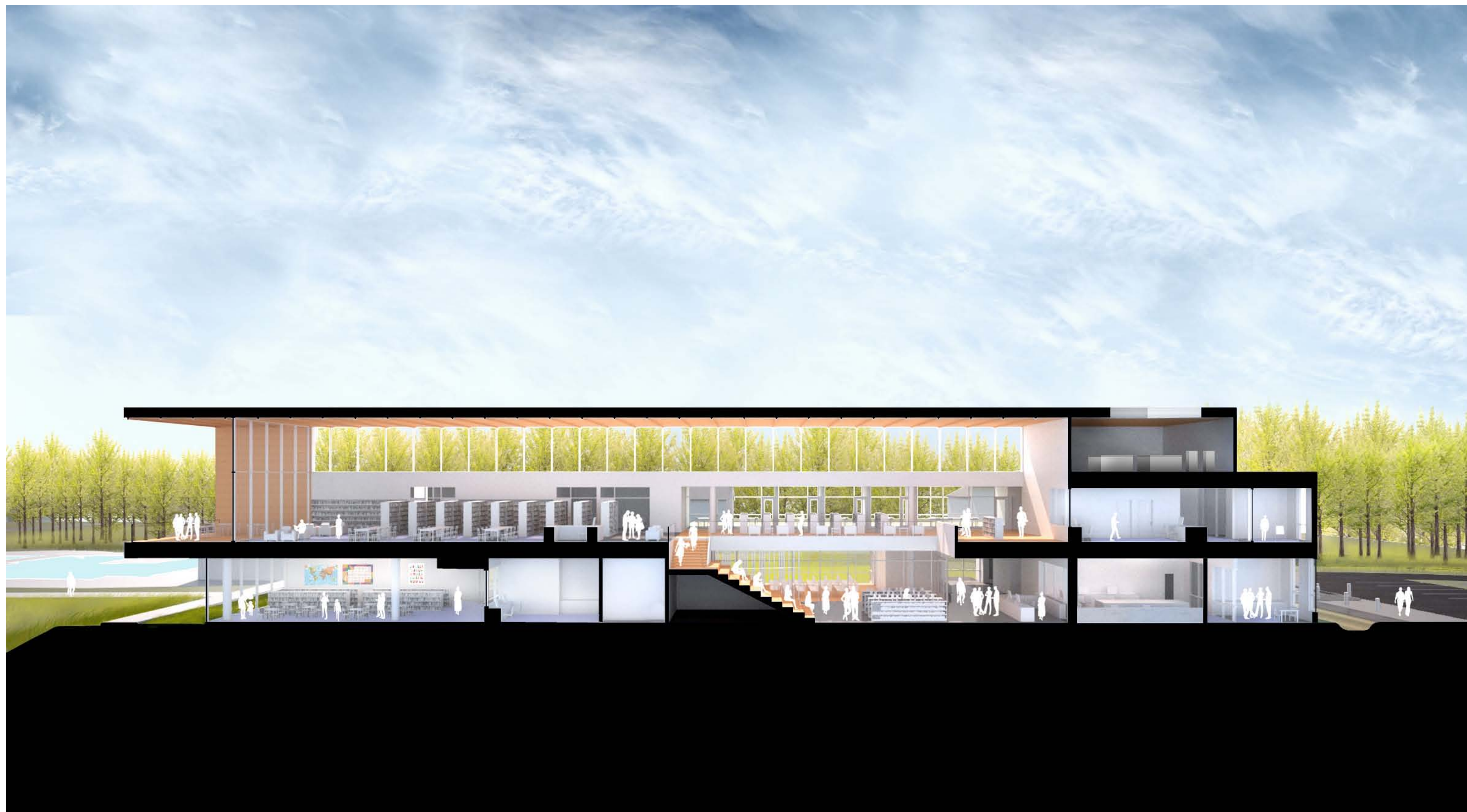
East-West Longitudinal Section
